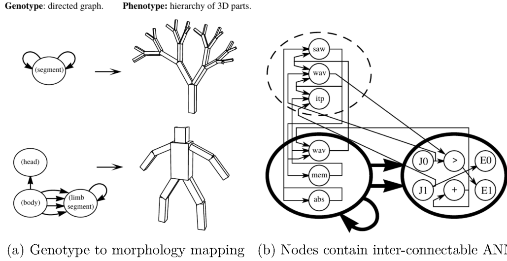
Figure 2.7: Overview of the different parts of a Graphtal: nodes contain morphological and neural data and links specify where each suborgan grow
