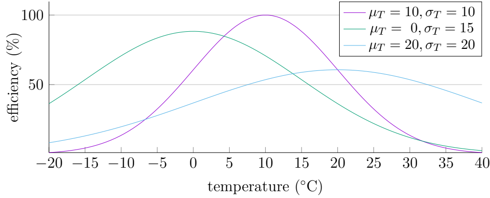
Figure 6.2: Samples of heat efficiencies for a handfull of parameters using, as in the following experiments m_{Tr} = s_{Tr} = 10^\circ\text{C} . One can see that, by favoring a larger range of acceptable temperatures, peak performance is conversely reduced.
