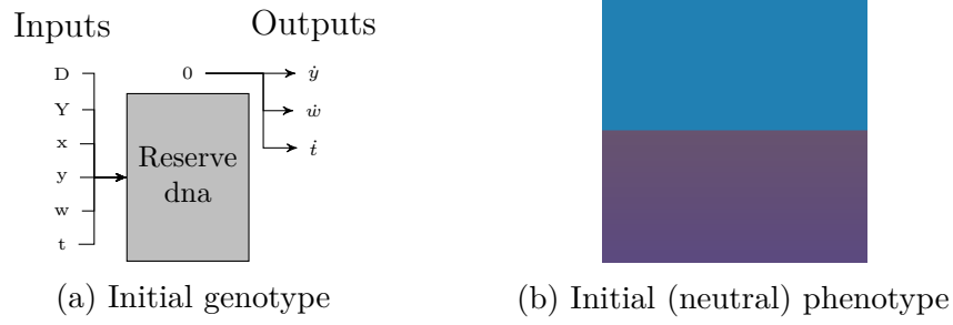
Figure 7.1: Initial state of the CGP (left) and resulting phenotype (right)
